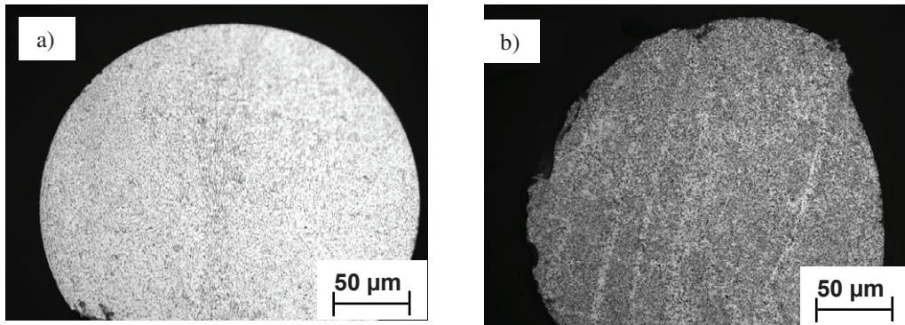
Figure 12: Optical micrographs of custom developed Al-Cu alloy on Al 6082 substrate after SLM processing (a) formation of single track of Al-2 wt. % Cu; (b) formation of single track of Al-5 wt. % Cu
