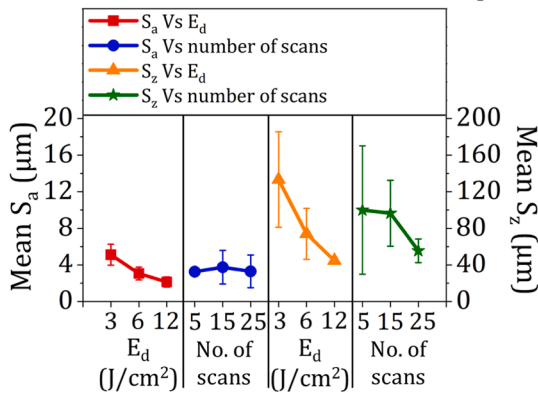
Fig. 4. Main effects of the LP parameters on mean S_a and S_z in Phase 1 experiments.
