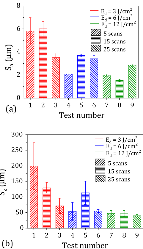
Fig. 3. (a) Average S_a and (b) average S_z calculated from the recorded surface roughness data at two locations of the LP surfaces in Phase 1 experiments.
