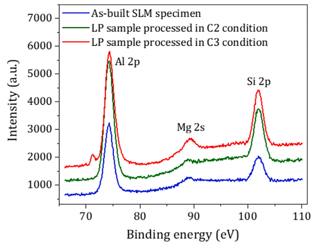
Fig. 14. XPS spectra obtained for the as-built SLM and LP specimens processed with 12 \text{ J/cm}^2 E_d and 10 scans in C2 and C3 conditions.
