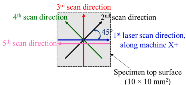
Fig. 2. Schematic diagram showing the change in the laser scan directions, covering the whole 10 \times 10 \text{ mm}^2 top surface: The first scan direction is along the machine X+ axis while each subsequent scan is given anti-clockwise at an angle of 45^\circ with the previous direction. The process is repeated for up to 25 scans.
