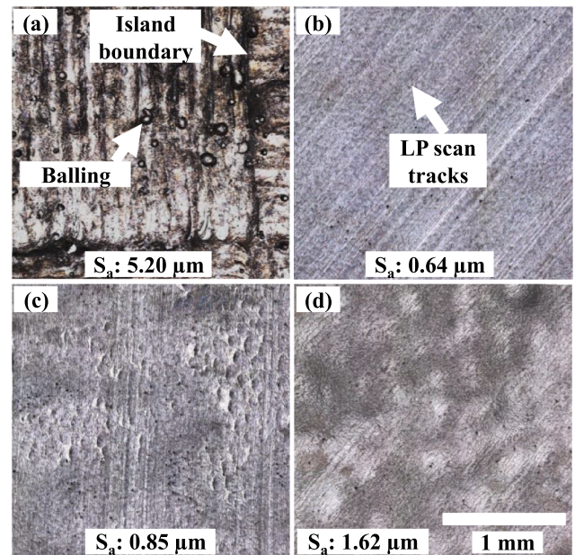
Fig. 7. Surface topographies of (a) an as-built SLM part; and specimens laser polished with 12 \text{ J/cm}^2 E_d and in (b) C2 condition with 10 scans; (c) C2 condition with 15 scans; and (d) C3 condition with 10 scans.
