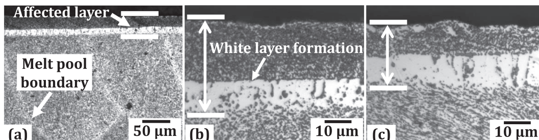
Fig. 12. Cross-sectional microstructures of LP specimens processed under (a), (b) C2 and (c) C3 conditions.
