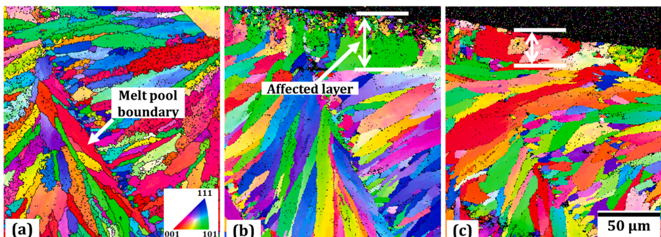
Fig. 15. EBSD inverse pole figures taken on the cross-sections of (a) an SLM specimen, and on cross-sections of LP samples processed in (b) C2 and (c) C3 conditions.
