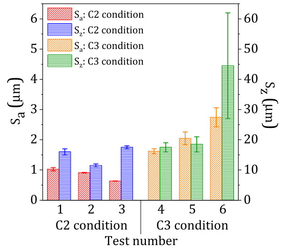
Fig. 6. Average S_a and S_z calculated from the recorded surface roughness data at two locations of the LP surfaces in Phase 2 experiments under air and argon environments, together with using the ceramic baseplate (C2 and C3 conditions, respectively).
