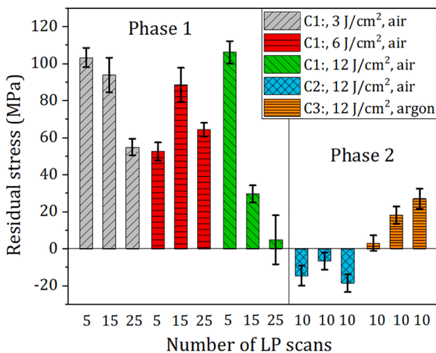
Fig. 9. Measured residual stresses on the parts laser polished under air and argon environments with and without the ceramic baseplate.
