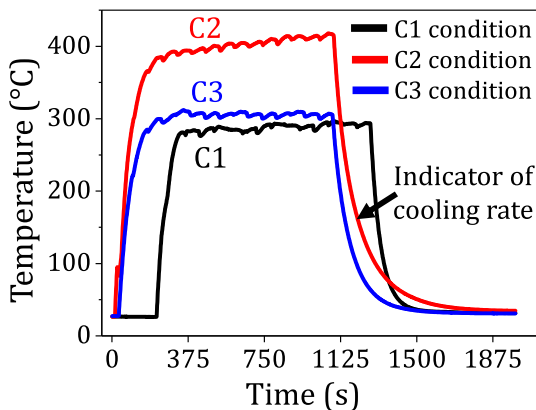
Fig. 5. Sub-surface temperatures recorded during and after LP with 12 \text{ J/cm}^2 E_d and 15 scanning passes.
