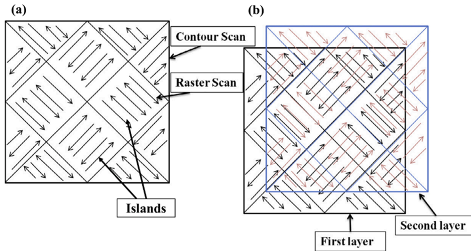
Fig. 1. Schematic illustration of the island scan strategy, showing (a) each layer is divided into squares (islands) and the inside of the island is raster scanned, then (b) the successive layers are displaced 1 mm in the X and Y-directions [29].
