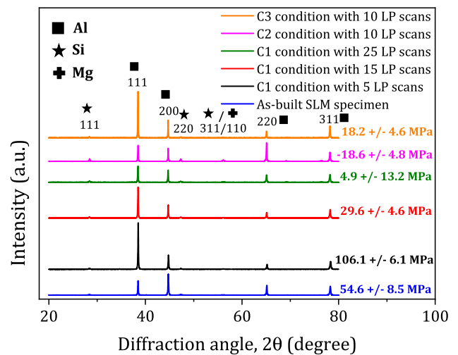
Fig. 10. Representative XRD spectra and the corresponding residual stresses for as-built SLM and LP specimens processed with 12 J/cm 2 energy density under C1, C2 and C3 conditions.
