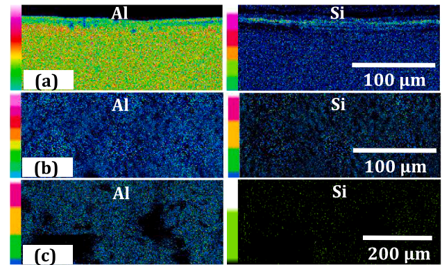
Fig. 13. EDS area mapping on the (a) cross-section of the LP specimen and (b) LP surface processed with 12 \text{ J/cm}^2 E_d and 10 scans under C2 condition; (c) as-built SLM surface.
