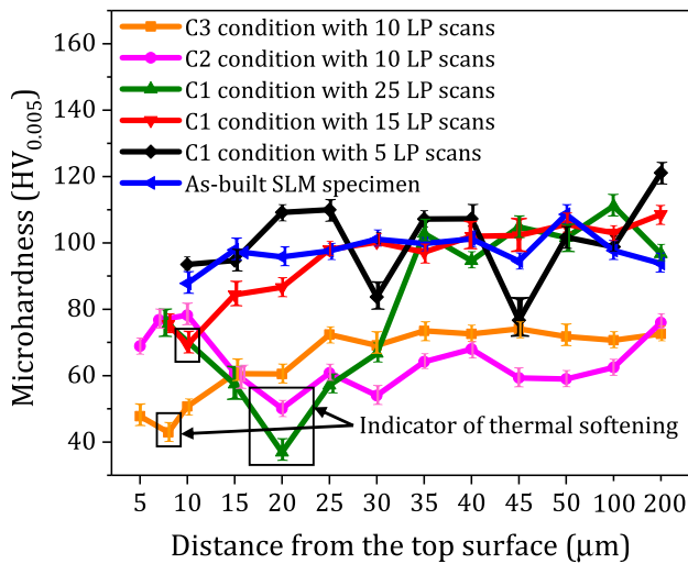
Fig. 11. Microhardness depth profiles for as-built SLM and LP specimens processed with 12 \text{ J/cm}^2 energy density and in air and argon environments with and without the ceramic baseplate.
