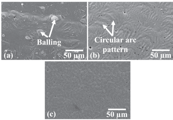
Fig. 8. SEM of (a) an as-built SLM surface; and surfaces laser polished with 12 J/cm 2 E d and in (b) C2 condition with 10 scans; and (c) C3 condition with 10 scans.
