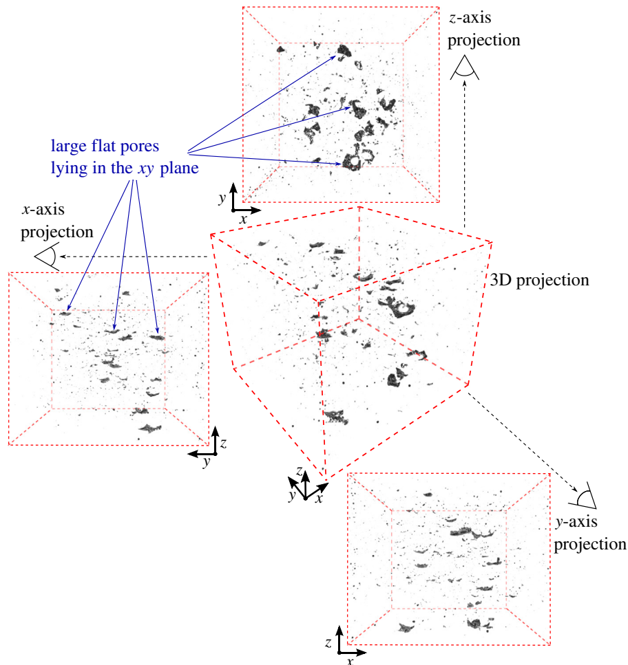
Fig. 12. {Pores (dark regions) in the SLM specimen, observed along the three principal axis and in 3D projection.}
