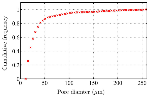
Fig. 8. Cumulative frequency (normalised to unity) of the pore diameters in the sample in its as-built condition.
