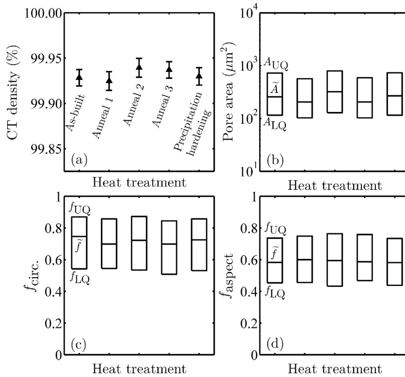
Fig. 9. Pore properties for the SLM specimen obtained after subsequent heat treatments (which are denoted in sub-figure (a) and described in Table 1. Mean CT densities are provided in (a). Median, upper quartile and lower quartile values for pore areas, circularities and aspect ratios are shown in (b), (c) and (d), respectively.
