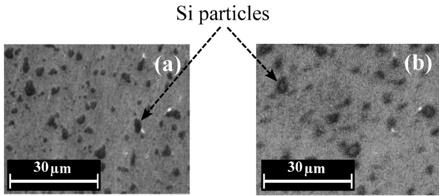
Fig. 15. SEM (a) and EDX (b) imaging of the SLM specimen in its final, precipitation hardened, state. The image presented in (b) shows EDX mapping in the same region as (a), obtained at the Si K\alpha_1 X-ray emission energy – the dark features are Si particles.
