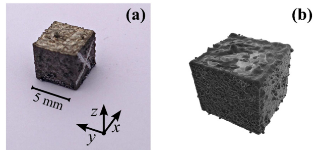
Fig. 1. Al–Si10–Mg SLM specimen selected for repeated CT measurements. (a) is a photograph, while (b) shows a three-dimensional reconstruction of the specimen from CT data.
