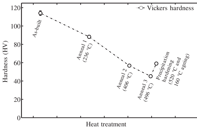
Fig. 16. Vickers hardness (HV) values obtained from multiple measurements of the SLM specimens under 300 gf (2.94 N) after subsequent heat treatments. The error bars of the last three data points are smaller than the symbols.
