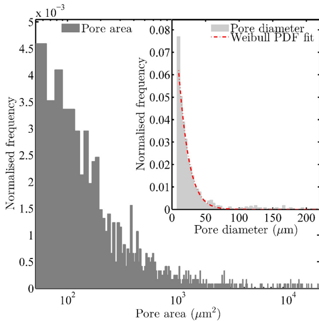
Fig. 7. Histograms representing the pore areas and (inset) diameters for the SLM specimen in the as-built condition. Also shown for the diameter distribution is the Weibull probability density function (PDF) fit.
