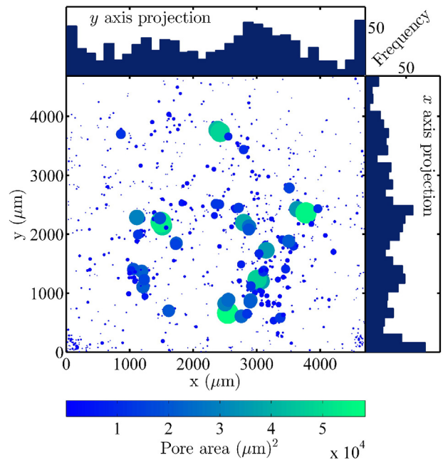
Fig. 6. All sampled pores in the SLM specimen projected onto a single xy plane. The relative point sizes are representative of each pore area, but they are not to scale. The data points are also coloured to indicate pore area. The x and y projected histograms represent pore numbers over the sampled volume.
