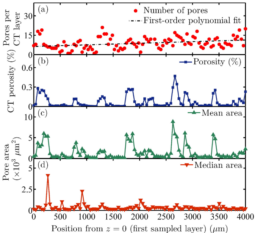
Fig. 4. Numbers of pores (a), porosity (b), mean (c) and median (d) pore areas at increasing height in the SLM specimen in its as-built condition.
