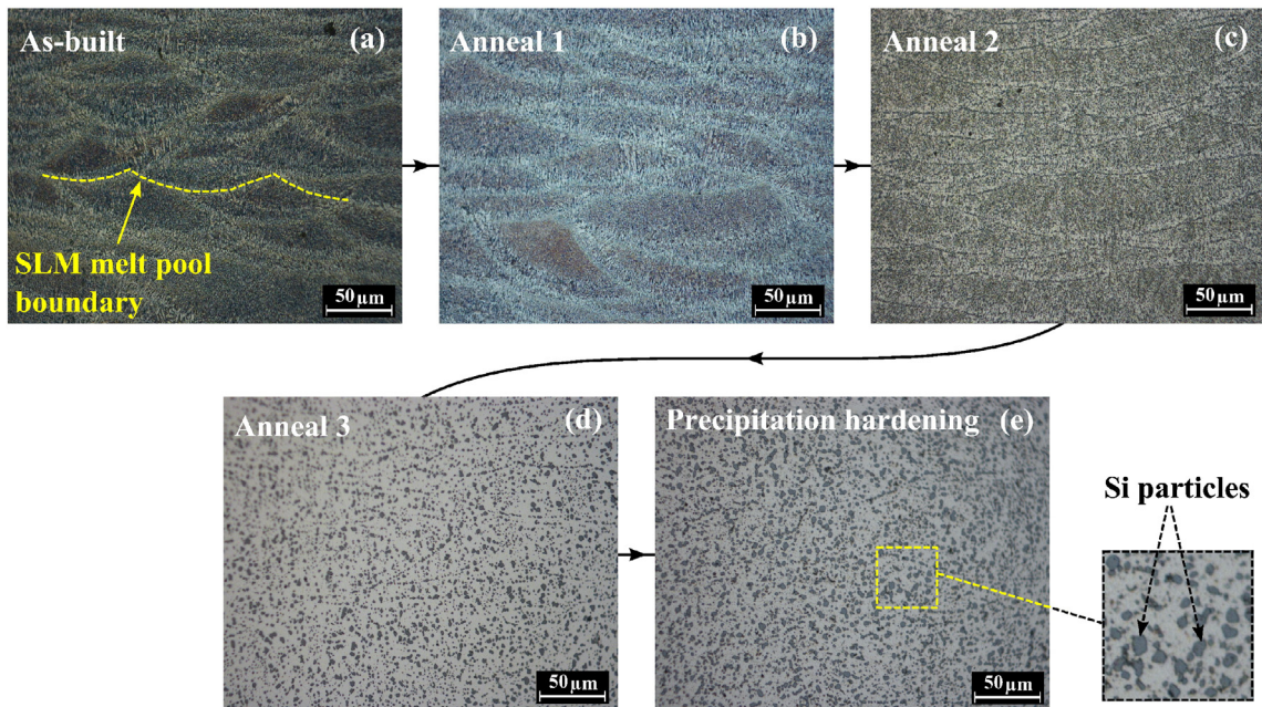
Fig. 14. Optical micrographs of polished and etched SLM specimens following subsequent heat treatments. Sub-figures (a) through (e) relate to the heat treatments described in Table 1. Regions of lighter and darker contrast are \alpha -phase Al and silicon particles, respectively.
