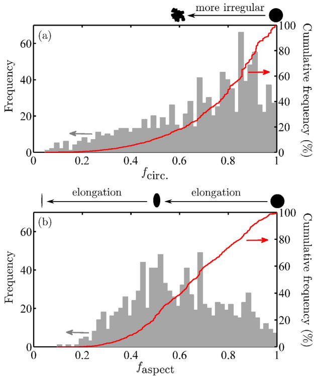
Fig. 10. Histograms and cumulative frequencies of circularity (a) and aspect ratio (b) of the pores in the as-built SLM specimen. These shape descriptors were defined in Eqs. (1) and (2), respectively.
