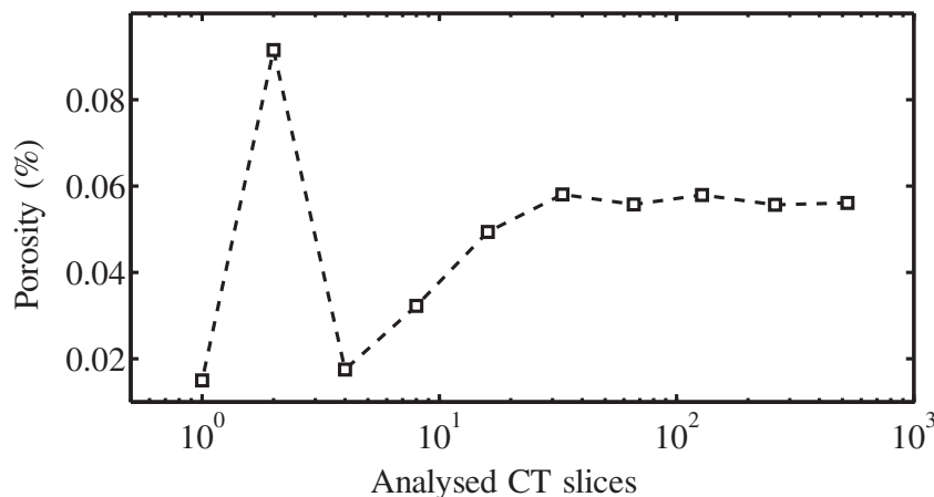
Fig. 2. Convergence of the total porosity with number of sampled CT slices.
