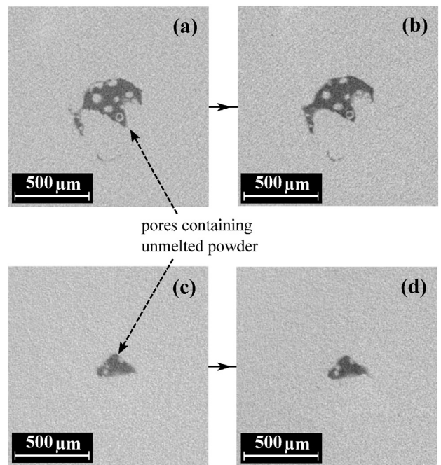
Fig. 11. Selected regions from a single CT slice of the SLM specimen in the as-built (a) and (c), and precipitation hardened (b) and (d), conditions. The pairs of sub-figures show the same pores, which contains some unmelted and unconsolidated powder (including one powder particle with an interior void).
