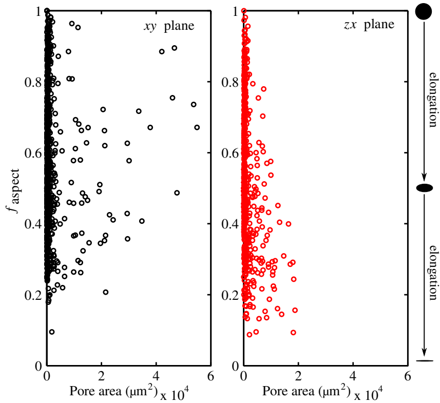
Fig. 13. Pore aspect ratios as a function of pore area for pores viewed in the xy plane (left) and zx plane (right).
