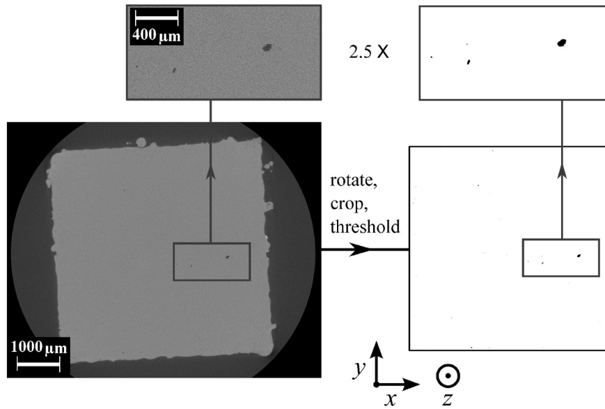
Fig. 3. The rotation, cropping and colour thresholding process used on each sampled CT layer allowing the porosity to be quantified.
