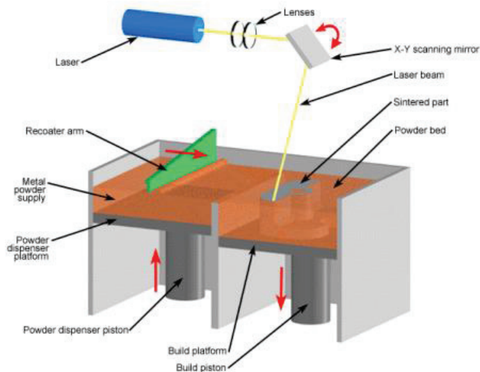
FIGURE 1. A schematic diagram of the AM powder bed technique machine
