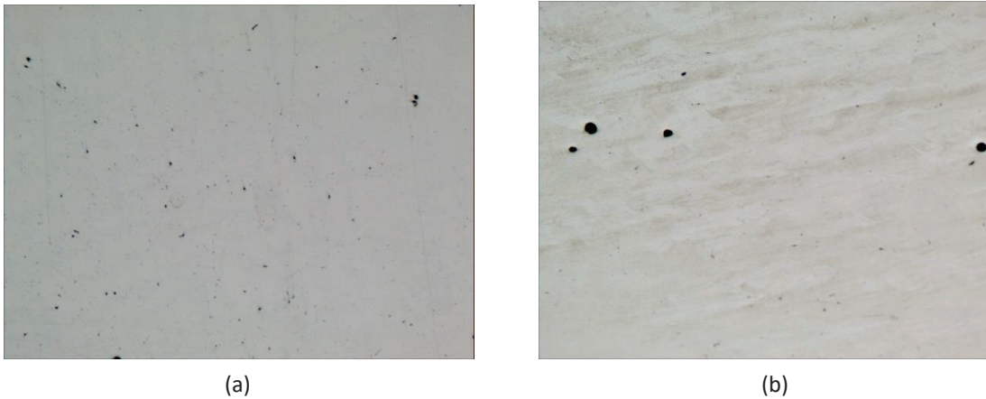
FIGURE 7. The porosity microstructure of the (a) top surface (b) side surface of sample 4.
