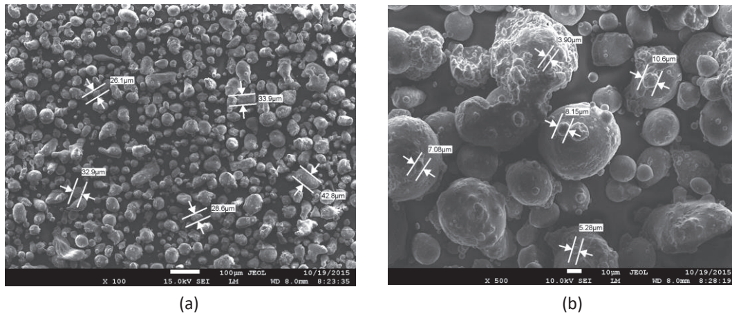
FIGURE 5. Field Emission Scanning Electron Microscope (FESEM, JSM-7600F) micrograph of AlSi10Mg powder (x100(a) & x500(b))
