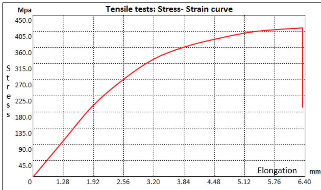
FIGURE 8. Stress-Strain curves for SLM AISi10Mg Samples built along X-Z direction
