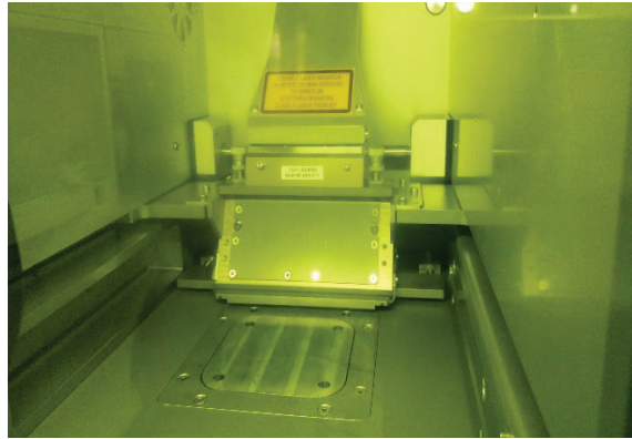
FIGURE 3. Build chamber SLM system SLM 125 HL
