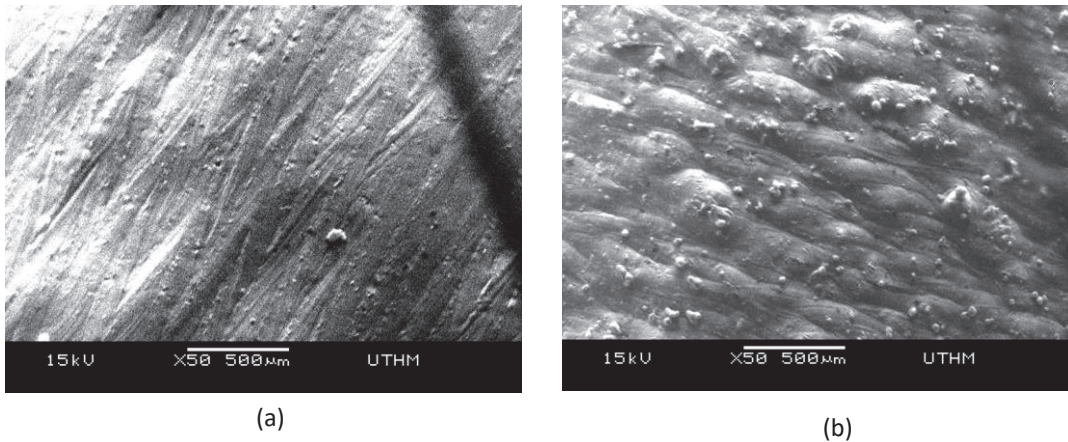
FIGURE 6. SEM micrograph of the (a) top surface (b) side surface of the AlSi10Mg samples by SLM (laser power: 350W; scanning speed: 1650 mm/s, hatching distance: 0.13 mm)
