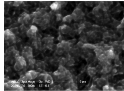
Fracture surface
