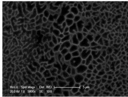
Dendritic micro structure
