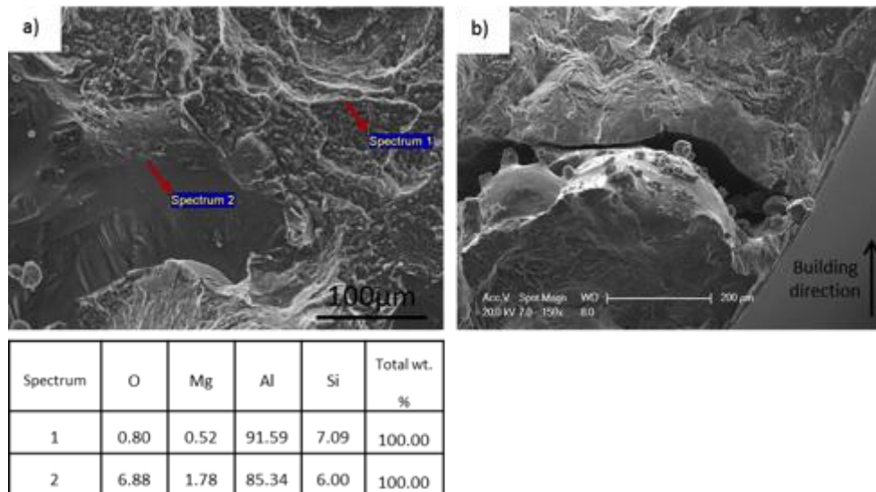
Fig. 13. Fractographs of the as-fabricated samples, showing (a) EDX on the fractured surface (spectrum 1), and on the black smooth void surface (spectrum 2), and (b) crack initiation site in a horizontally built and machined sample, void cut open to the surface.
