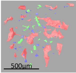
Voids in as-fabricated build ( \mu CT)
